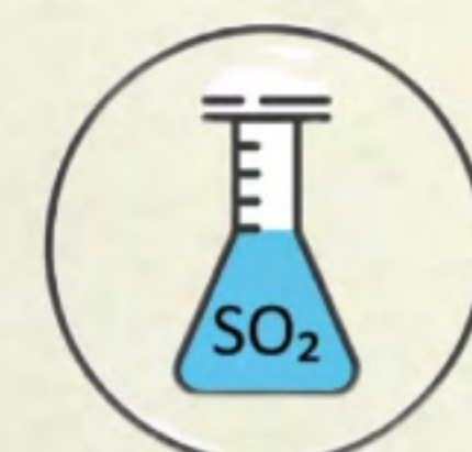
SULPHUR DIOXIDE
